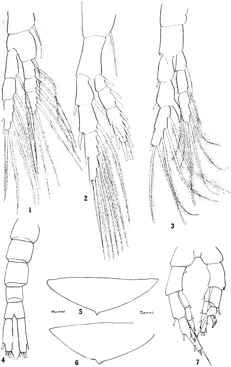
1-3. Limnocalanus macrurus : 1, First swimming foot; 2, second swimming foot; 3, fifth foot of female. 4-7. Limnocalanus johauseni : 4, Abdomen of male; 5, 6, last thoracic segments; 7, fifth feet of male.
